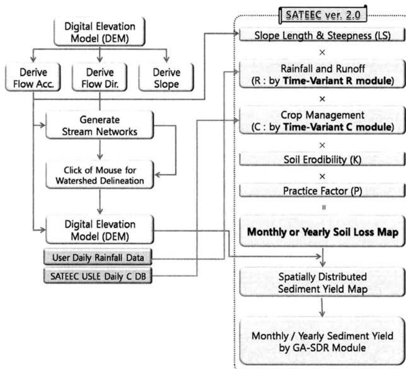
Fig. 1. Overview of the SATEEC System ver. 2.0 (Park et al., 2010).
