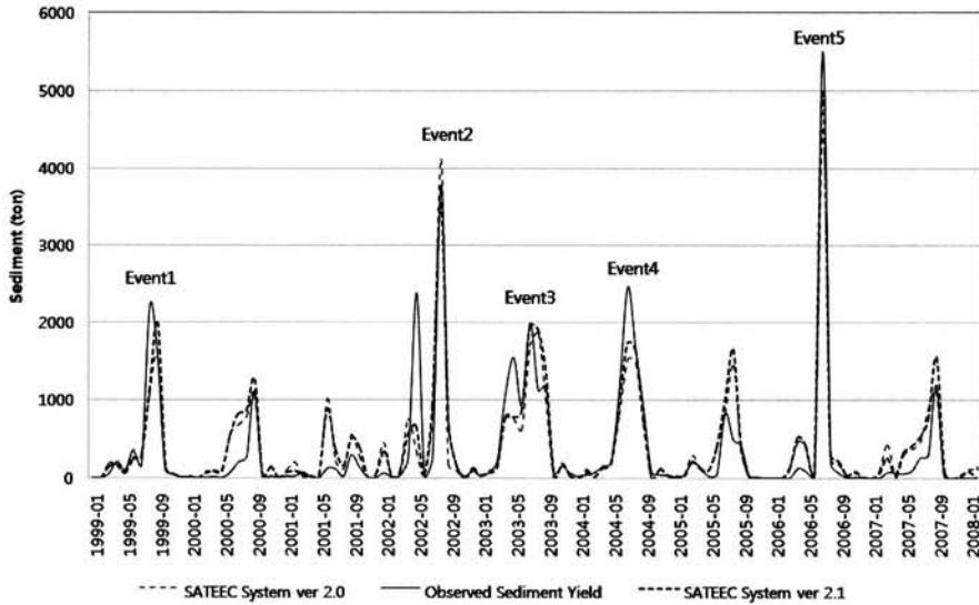
(a) Sediment yield (1999 ~ 2008)
