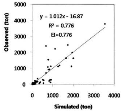
(c) R^2 and EI of simulated sediment yield by SATEEC system ver. 2.1
