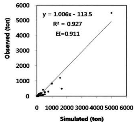
(c) R 2 and EI of simulated yield by SATEEC system ver. 2.1.
