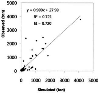
(b) R^2 and EI of simulated sediment yield by SATEEC system ver. 2.0
