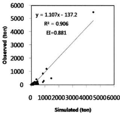
(b) R 2 and EI of simulated yield by SATEEC system ver. 2.0
