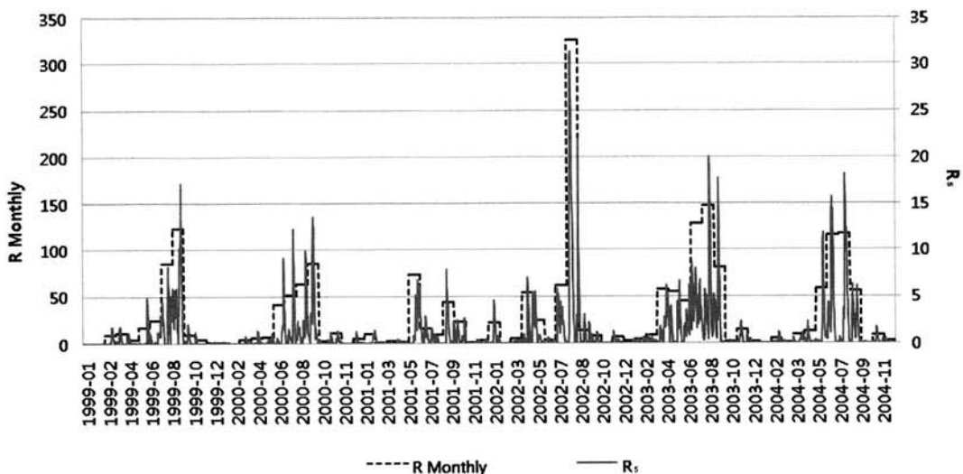
Fig. 4. Comparison of R monthly and R 5 .
