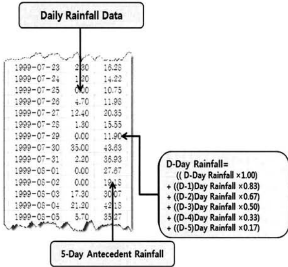
Fig. 2. Estimation of '5-Day Antecedent Rainfall'.
