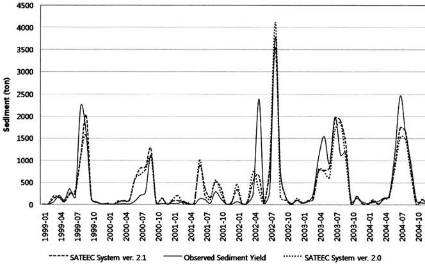
(a) Comparison of observed sediment yield, simulated sediment yields by SATEEC system ver. 2.0 and SATEEC system ver. 2.1
